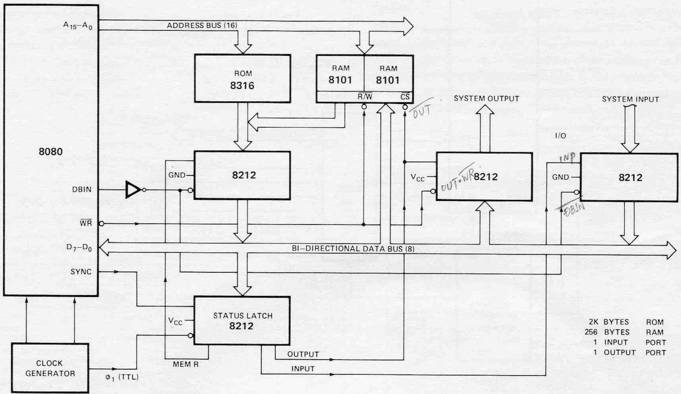
Figure 5. Minimum 8080 System.
