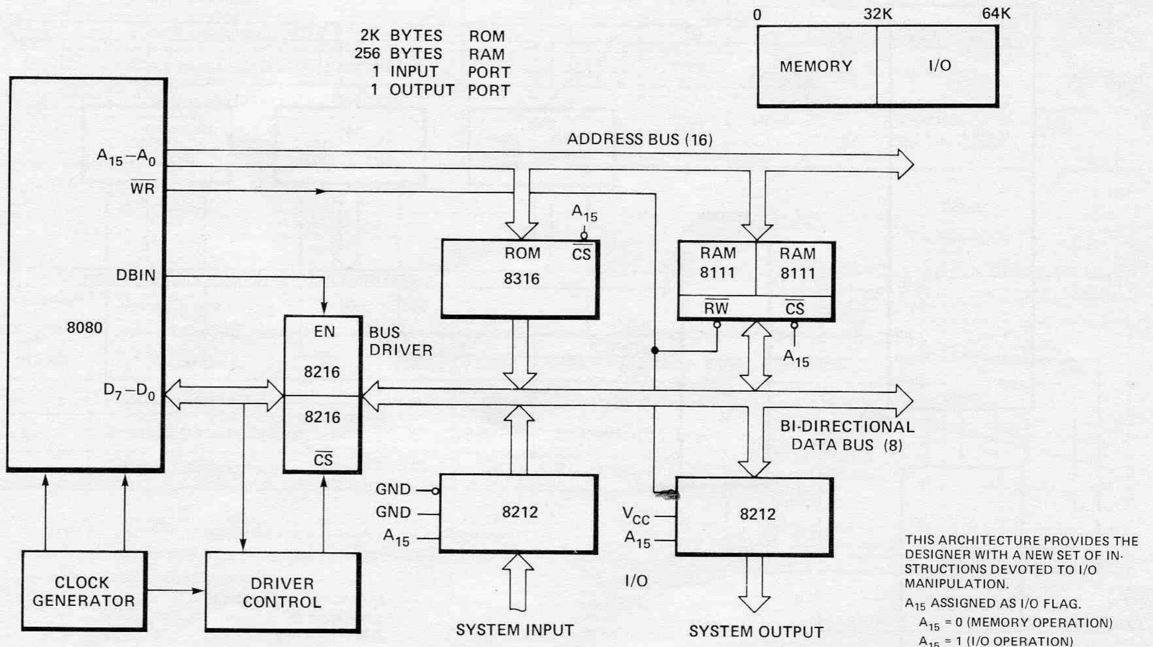
Figure 6. Minimum 8080 System (MEMORY MAPPED I/O).
