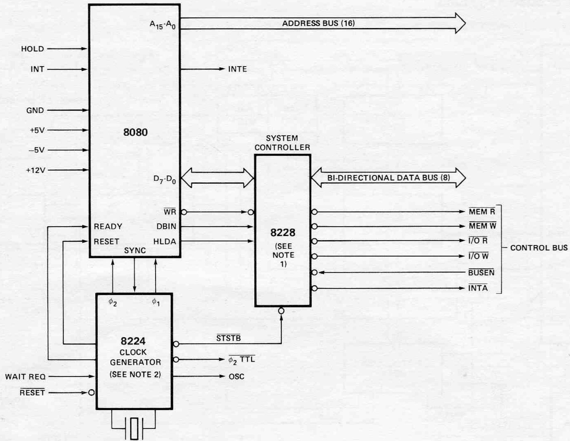
Figure 7. 8080 Standard Interface.
