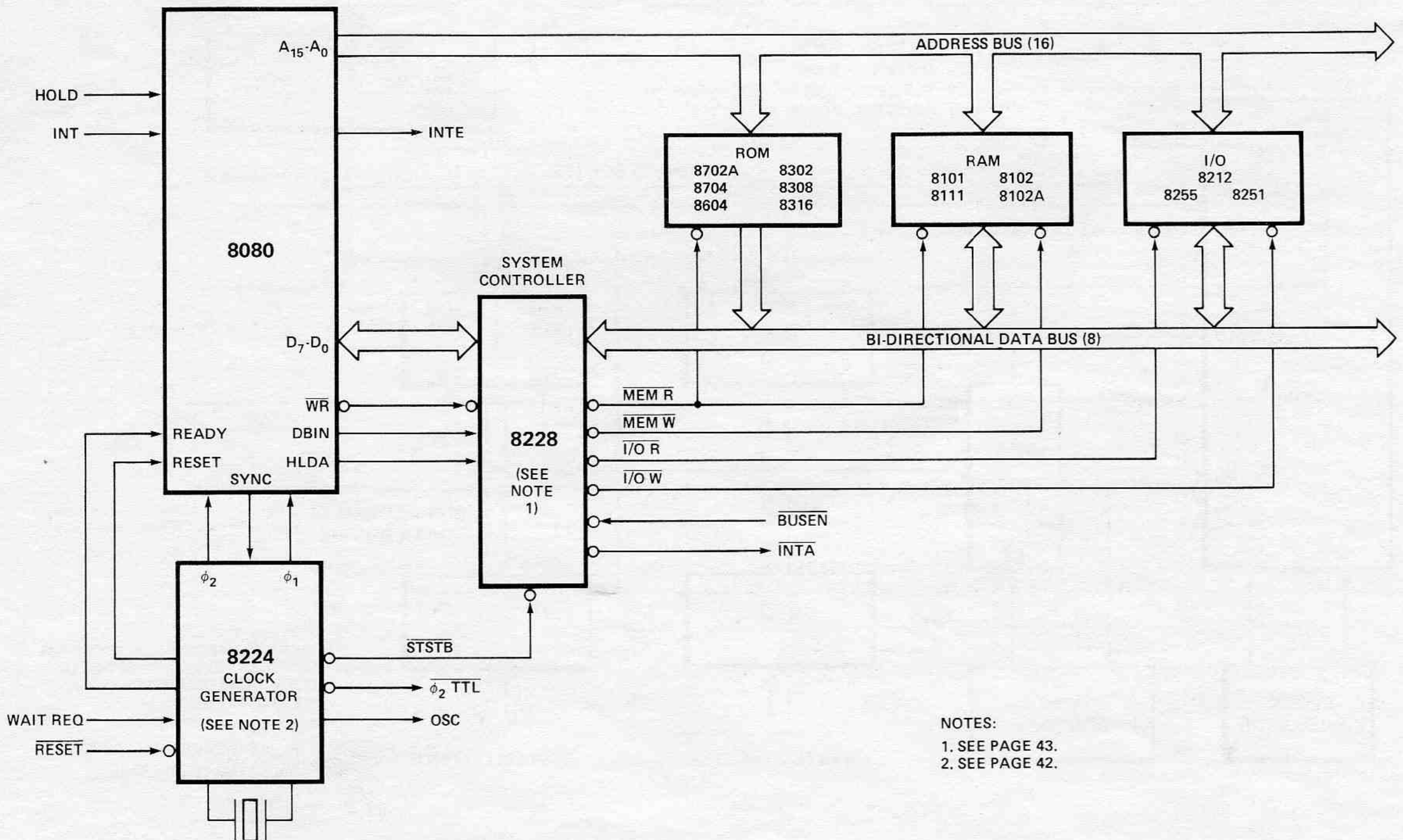
Figure 8. 8080 Standard System Architecture.
