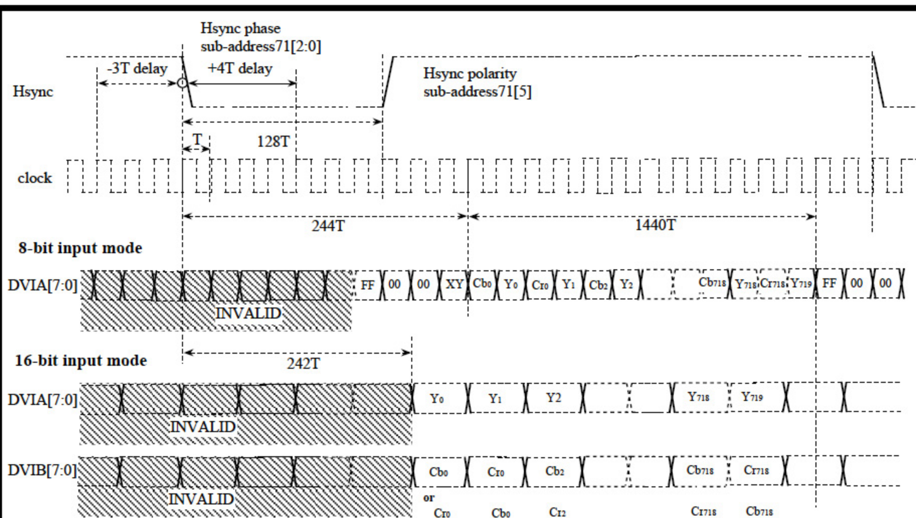
Fig 3 : Digital Input Timing(525/60 system) in Master Mode
